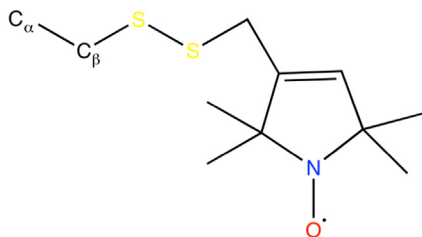
FIGURE 1 Schematic of MTSL. MTSL is a commonly used PRE tag because of its sulfhydryl specificity and side-chain flexibility. The oxygen atom is the paramagnetic center. To see this figure in color, go online.
