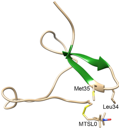
FIGURE 4 Representative configuration of the MTSL-Cys-A \beta 42 ensemble, showing increased side-chain interactions between MTSL-Cys and Leu34 and Met35, which contributes to a more collapsed structural ensemble and \beta -strand pairings (darker shade) between residues 29–32 and 36–38. This new \beta -structure is present in negligible amounts in the untagged peptide. Chimera ((73); University of California, San Francisco) was used to generate the molecular graphics. To see this figure in color, go online.
